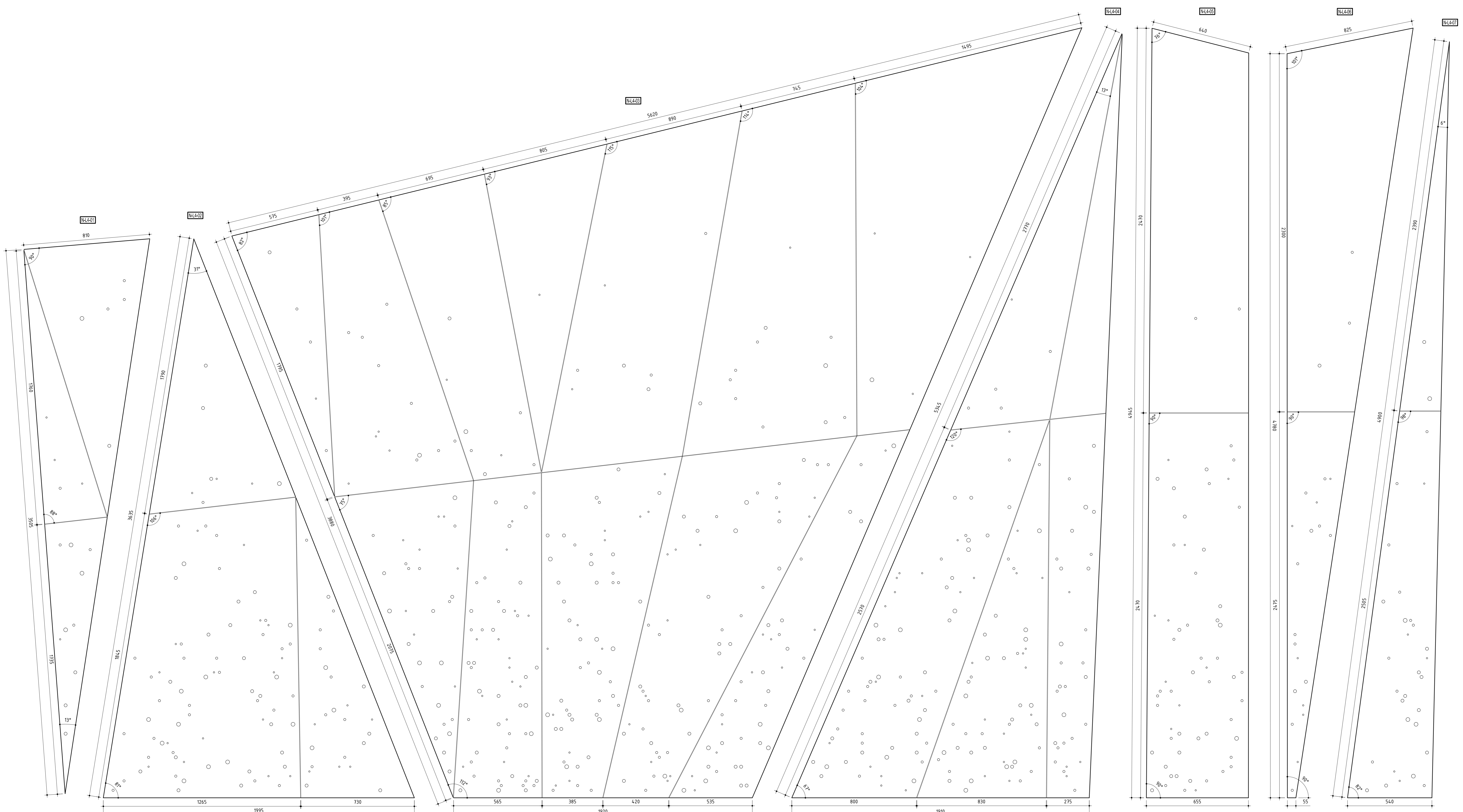
01 UNFOLDED PANELS: N-L4-01 THROUGH N-L4-07 SCALE: 1:10
